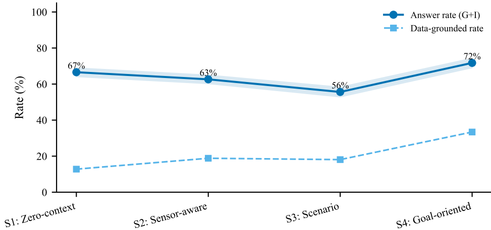
Answer rate across elicitation stages ( V=0.12 , p=0.000 )
